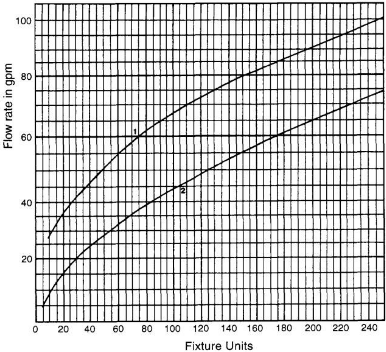
Figure 4.2: Enlarged Scale Demand Load estimation Curve
