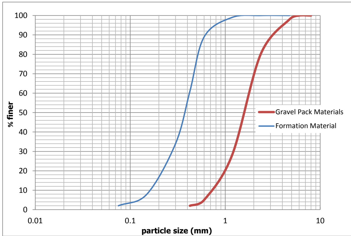
Figure: Typical Gradation Curve of gravel pack materials
