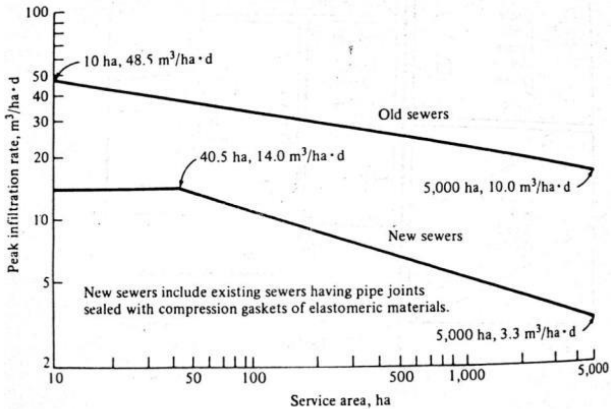
Figure 5.4: Peak infiltration rates for residential areas[3]
