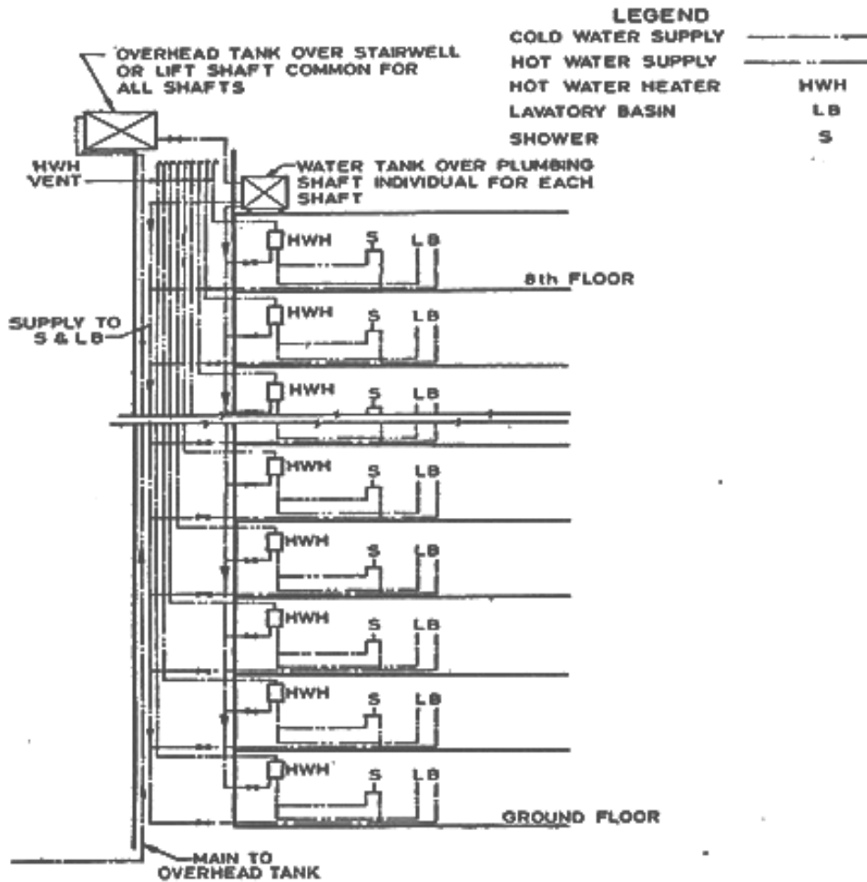
Figure 4.4: Layout plan of the water supply system of a tall building
