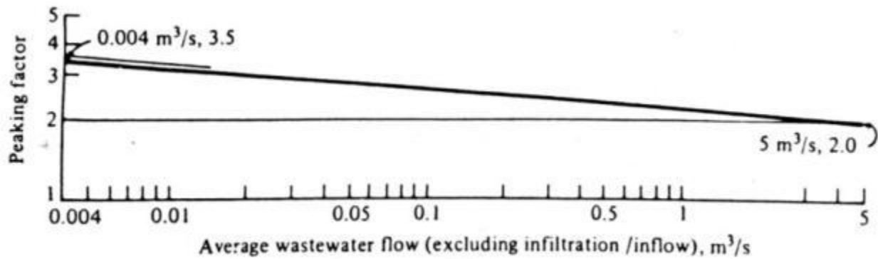
Figure 5.5: Peak factor for residential areas[3]
