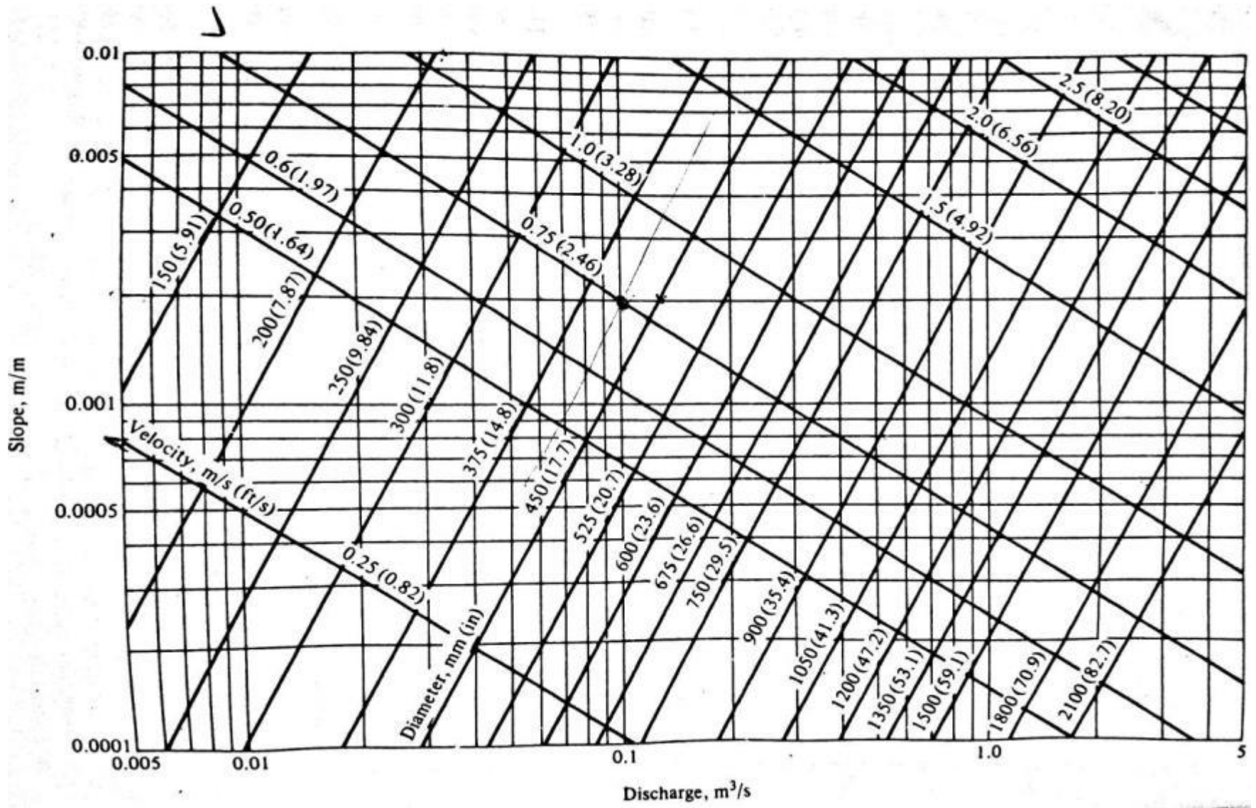
Figure 5.2: Graphical presentation of manning's equation for n = 0.013 [3]
