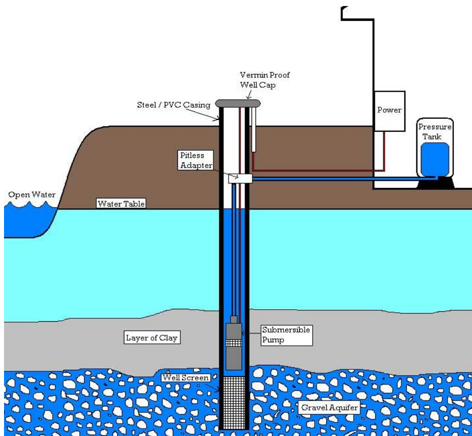
Figure 3.1: Elements of a production well
