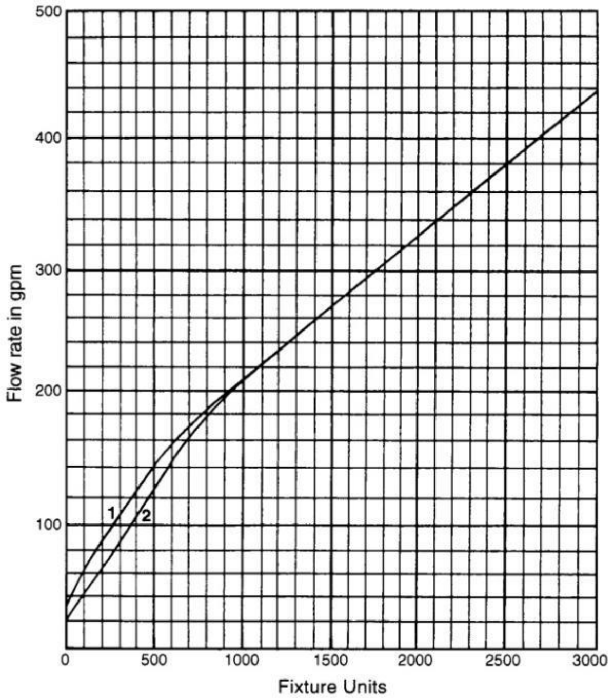
Figure 4.1: Estimate Curve for Demand Load
