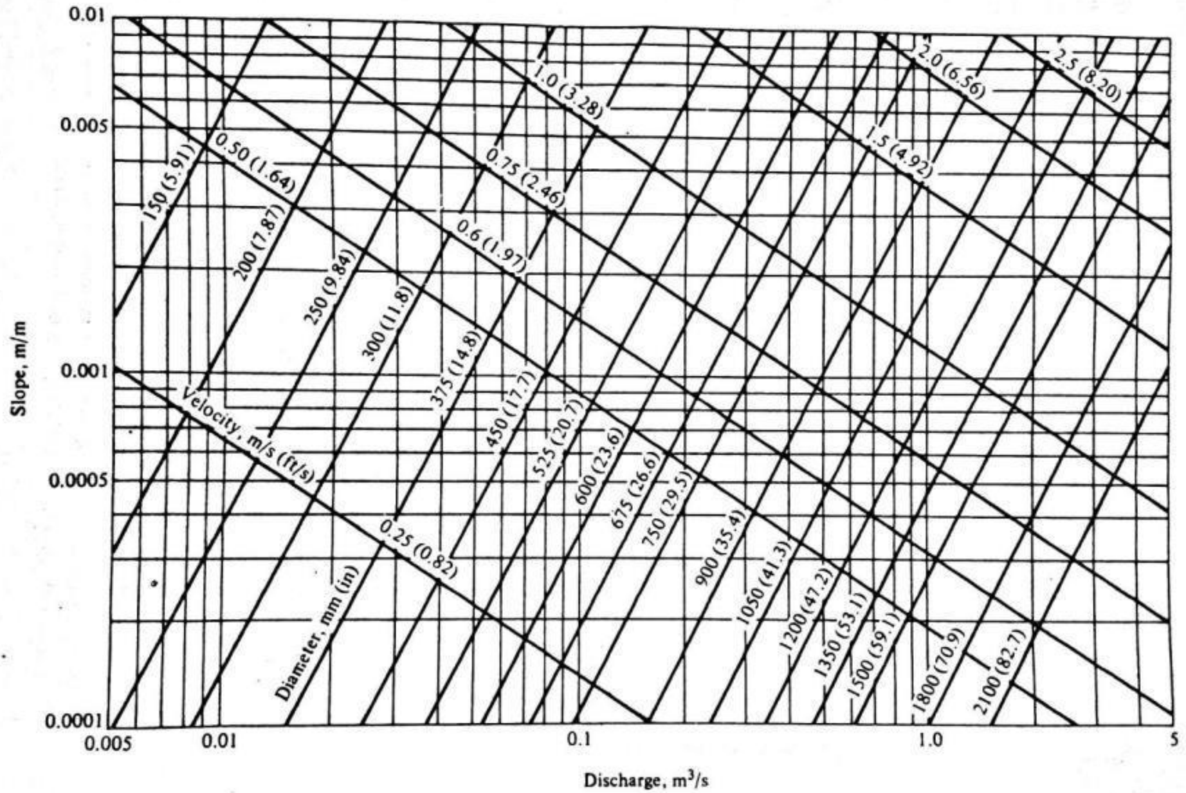
Figure 5.3: Graphical presentation of manning's equation for n = 0.015 [3]
