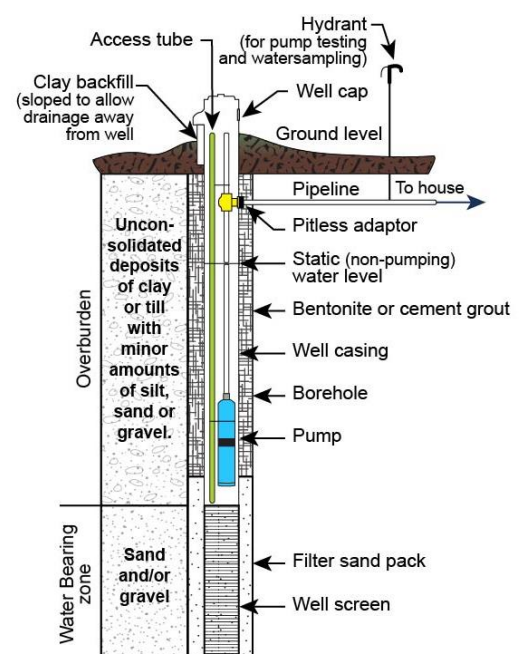
Figure 3.2: Gravel Packed Well
