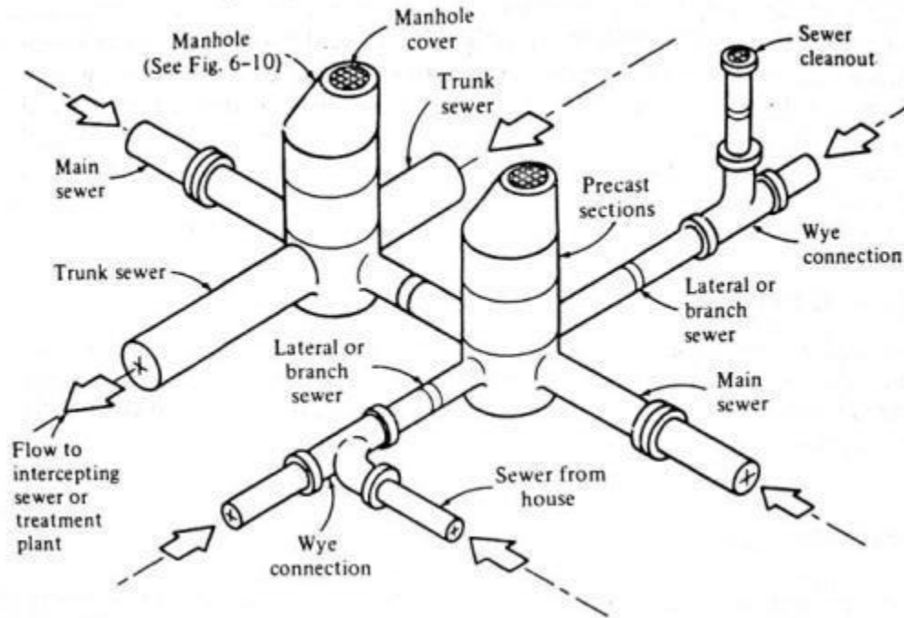
Figure 5.1: Definition sketch for types of sewers[3]
