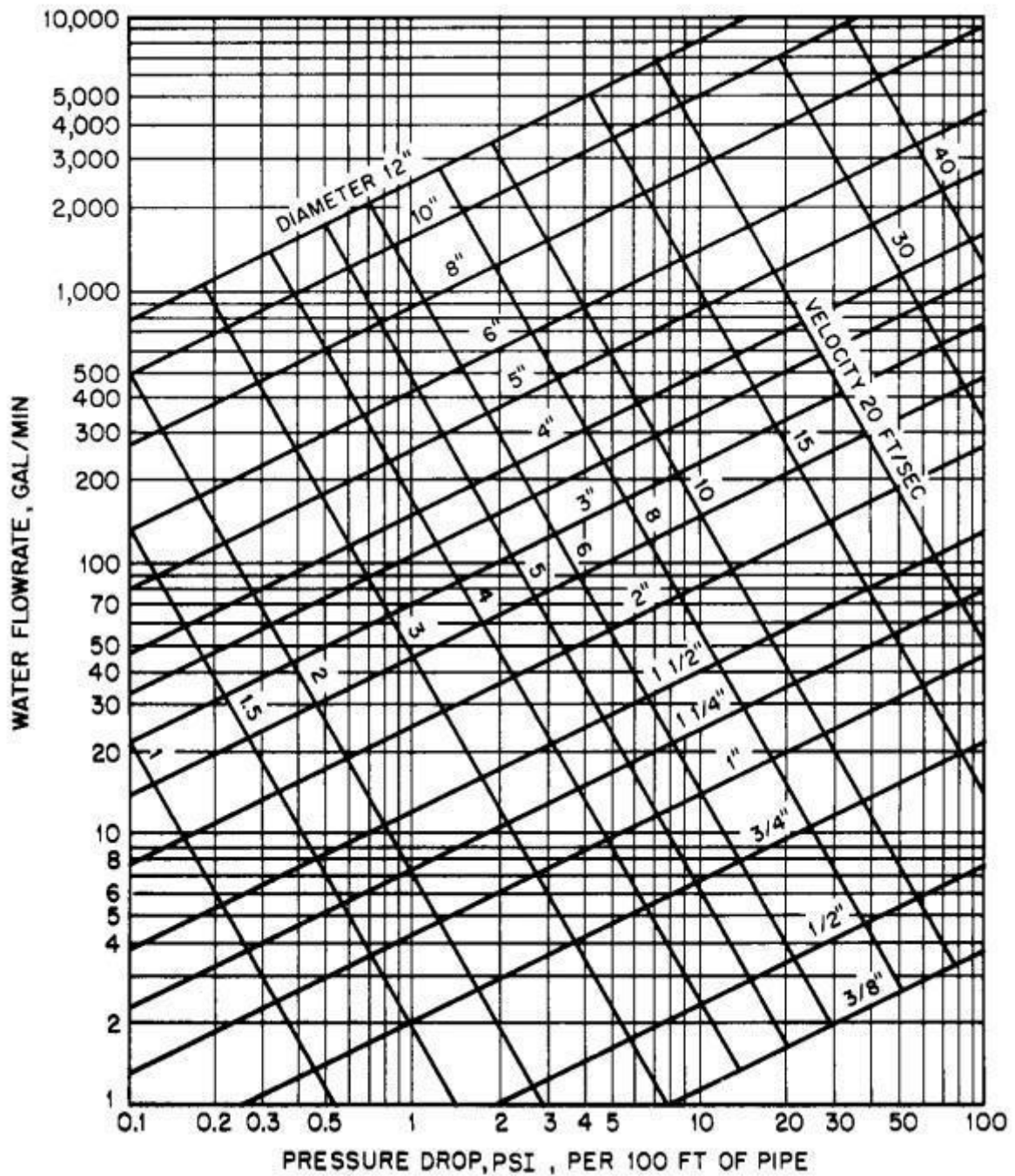
Figure 4.3: Chart for determination of flow in pipes such as galvanized steel and wrought iron that will be fairly rough after 15 to 20 years of use [2]
